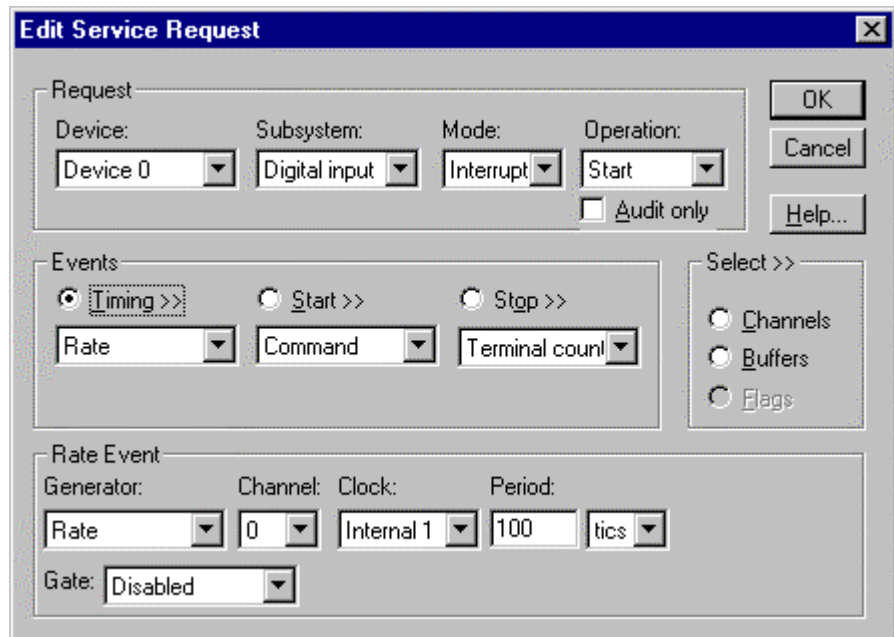
How to set up the KPCI-PIO for fixed rate sampling using an internal clock.
