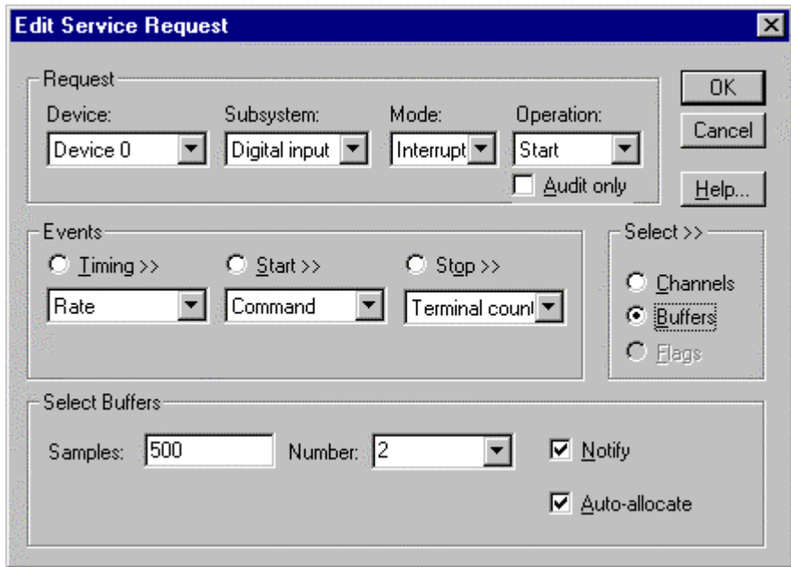
How to set up the KPCI-PIO to read digital samples using data buffers
