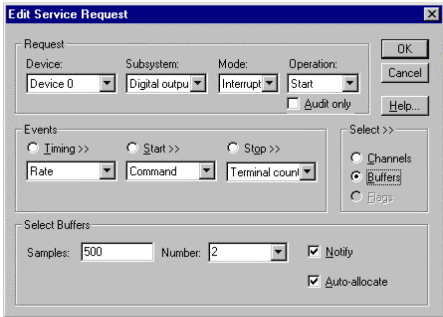
How to set up the KPCI-PIO to write digital samples using data buffers
