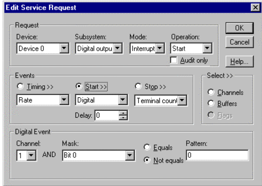
How to set up the KPCI-PIO for post-triggered digital output.
