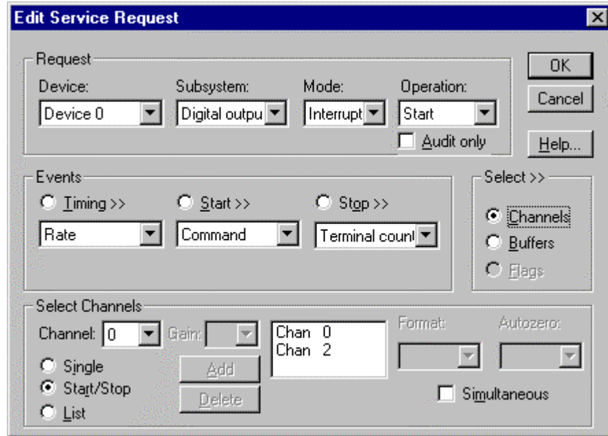
How to set up the KPCI-PIO to write from a range of channels
